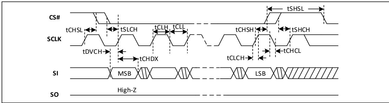
Figure-78. Serial Input Timing (DTR mode)
