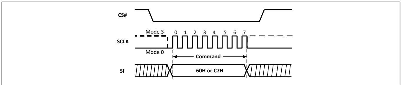
Figure-41. Chip Erase Sequence Diagram
