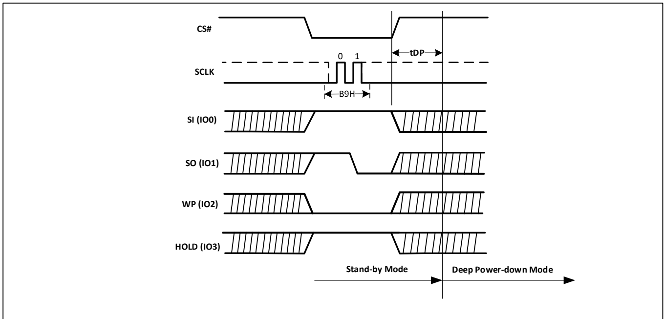
Figure-50. Deep Power-Down Sequence Diagram (QPI)
