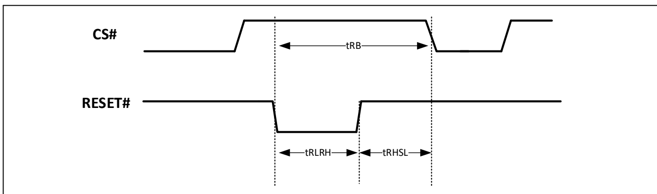
Figure-84. RESET Timing
