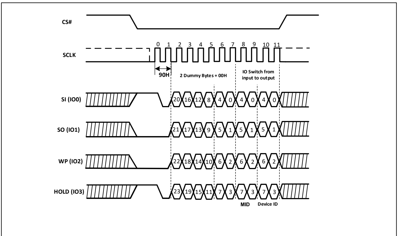
Figure-56. Read Electronic Manufacturer ID & Device ID Sequence Diagram (QPI)
