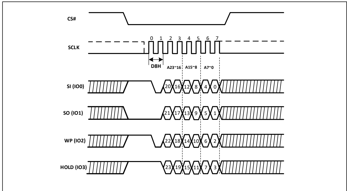
Figure-40. Block Erase Sequence Diagram (QPI)
