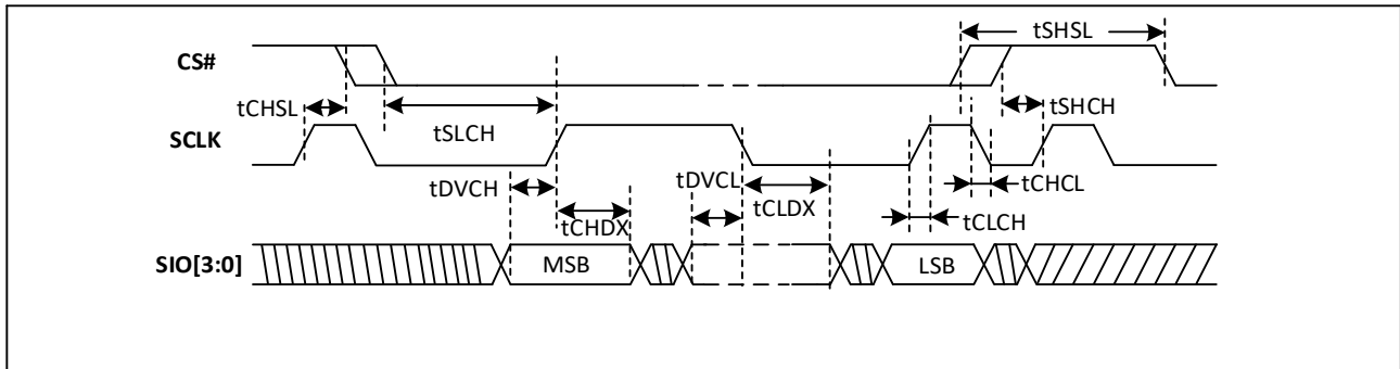
Figure-79. Output Timing
