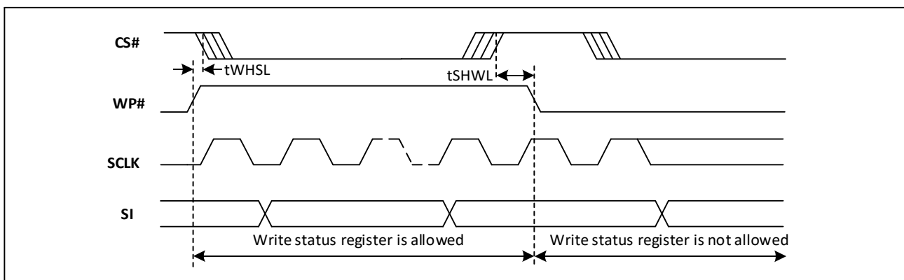
Figure-83. Resume to Suspend Timing Diagram
