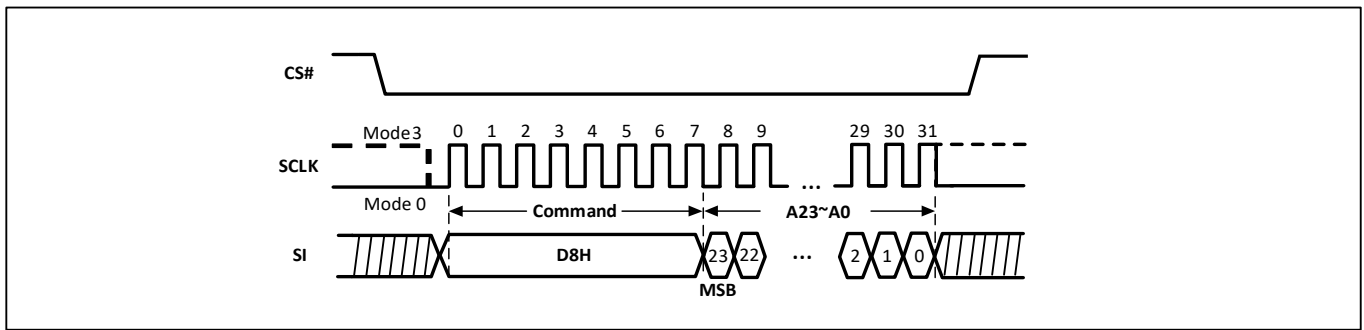
Figure-39. Block Erase Sequence Diagram
