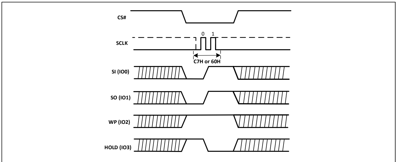
Figure-42. Chip Erase Sequence Diagram (QPI)
