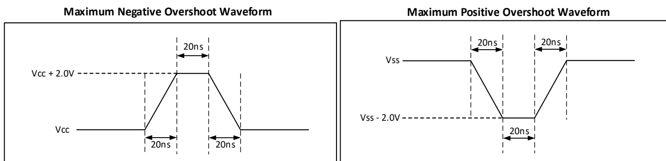
Figure-74. Maximum Negative/positive Overshoot Diagram
