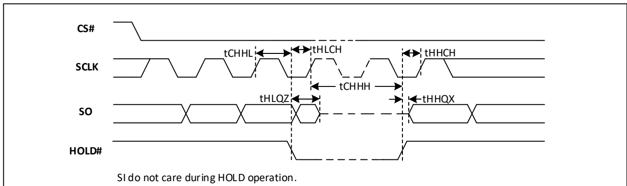
Figure-81. Hold Timing
