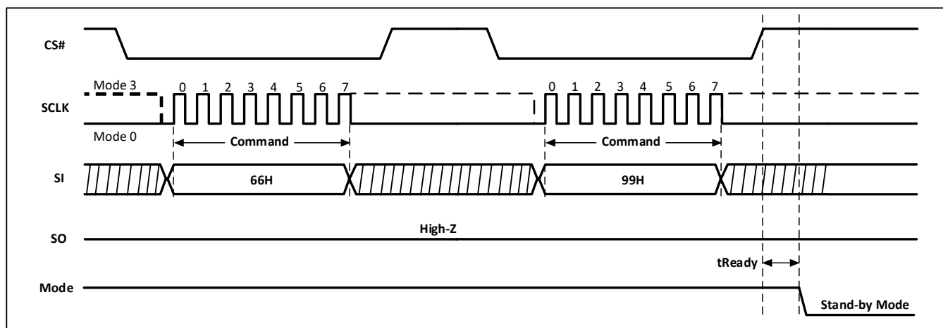
Figure-69. Reset Enable and Reset Sequence Diagram
