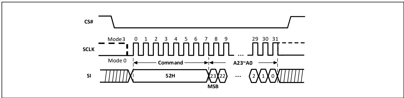
Figure-37. Half Block Erase Sequence Diagram
