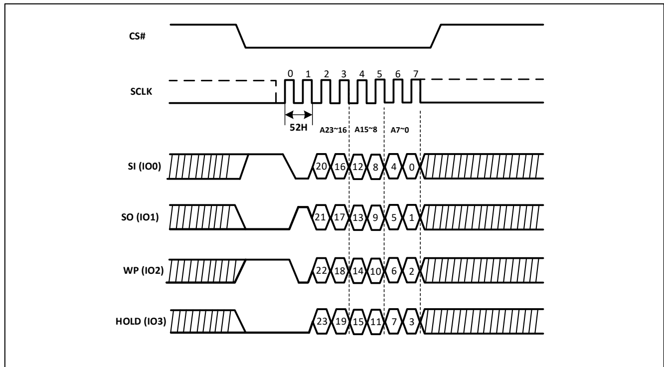
Figure-38. Half Block Erase Sequence Diagram (QPI)
